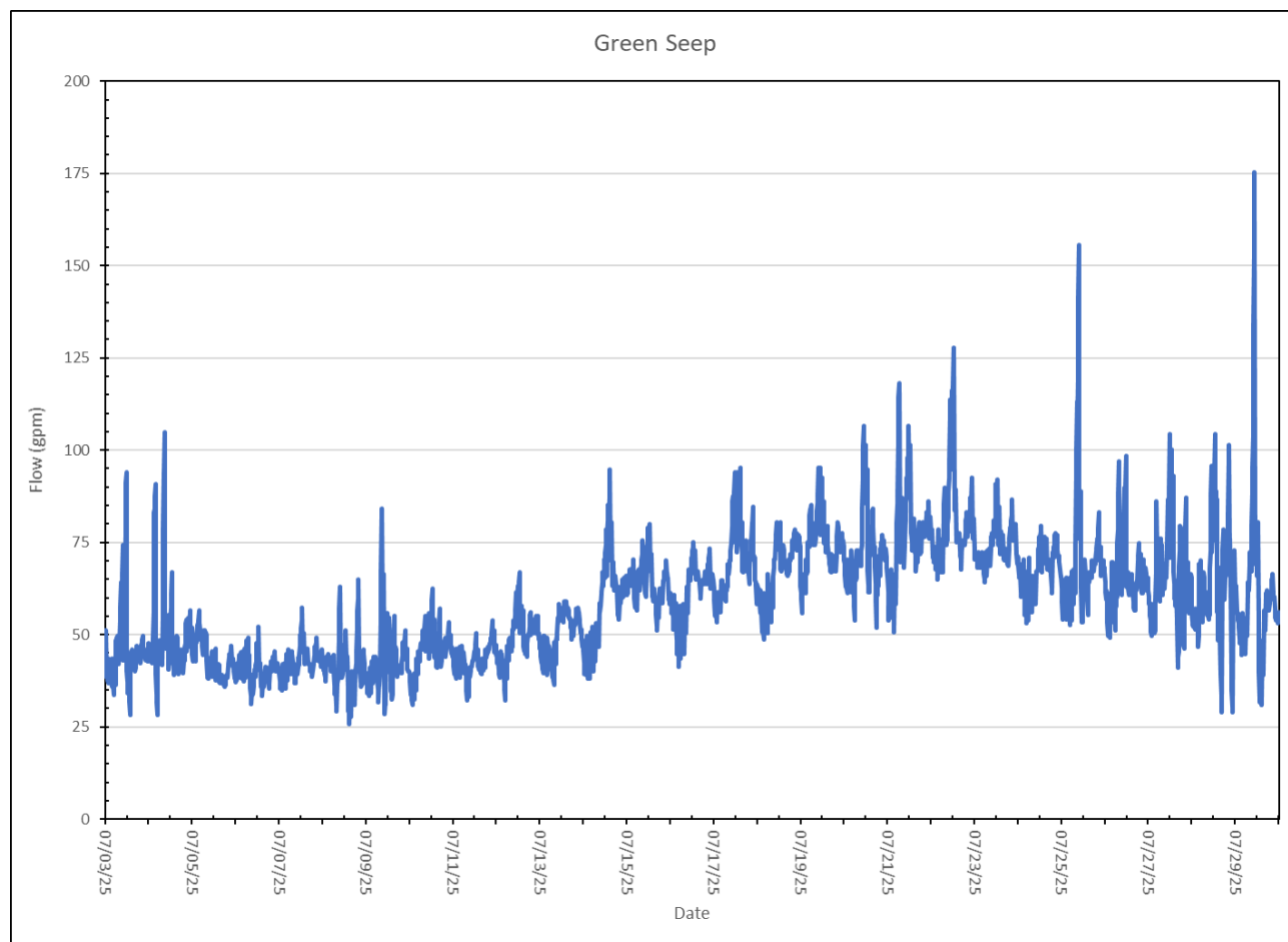
Figure 7. Green Seep flow rate, July 2025.
