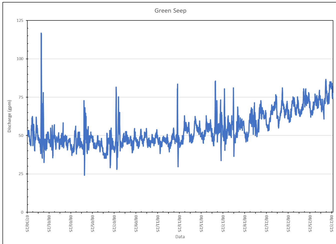
Figure 7. Green Seep flow rate, August 2025.
