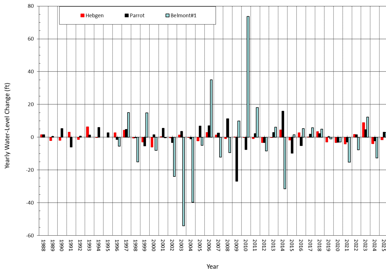
Figure 3-18. Park wells annual water-level changes.
