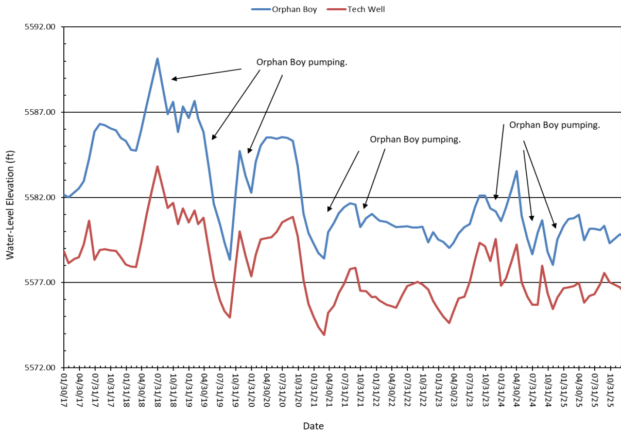
Figure 5-3. Hydrographs from the Orphan Boy and Montana Tech wells show the influence of 2018–2025 Orphan Boy pumping events and monthly water-level readings, 2017–2026.
