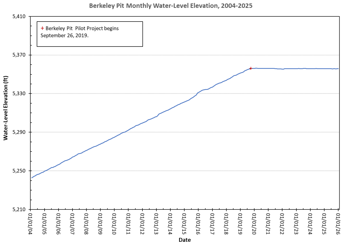
Figure 6-1. Berkeley Pit water-level elevation from 2004 through 2025. The Horseshoe Bend water-treatment plant came online in late 2003 and Horseshoe Bend water was no longer allowed to flow into the Berkeley Pit. The beginning of the Berkeley Pit Pilot Project is also shown.
