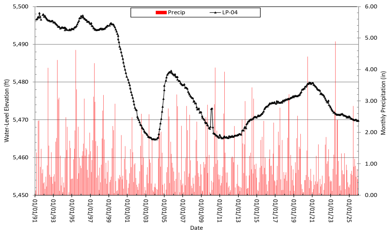
Figure 2-11. Hydrograph for well LP-04 located north of the Pittsmont Waste Dump and south of the leach pads.
