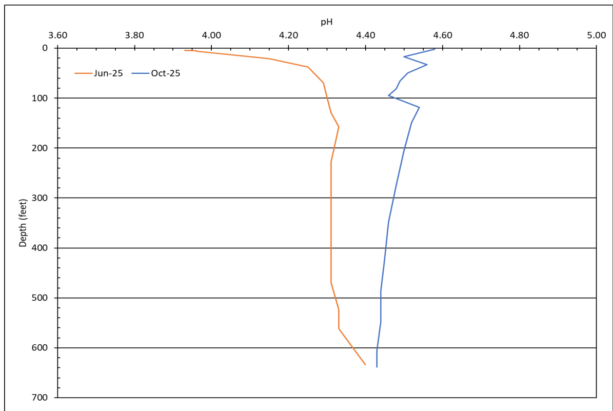
Figure 3-31. Berkeley Pit 2025 pH profiles.
