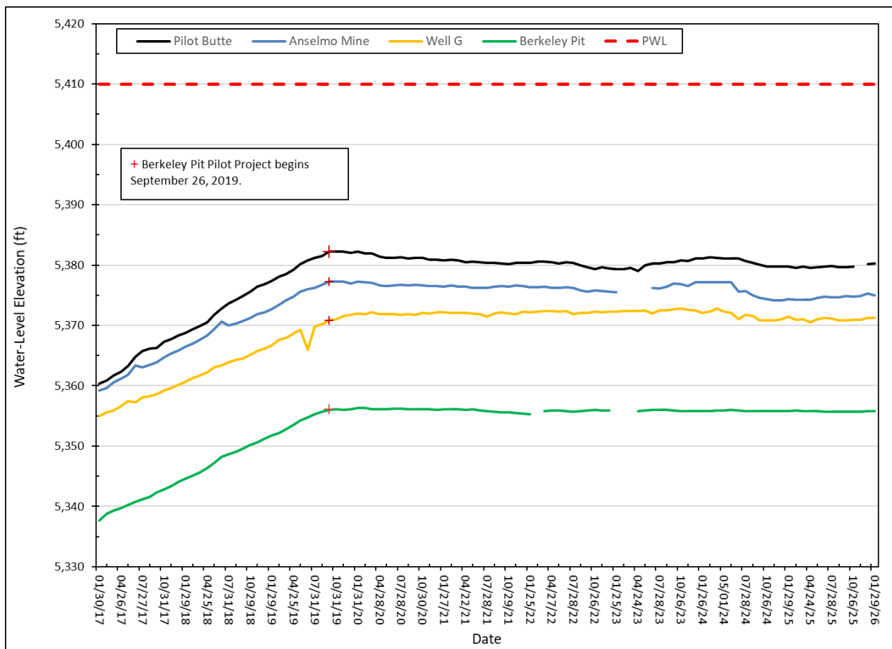
Figure 3-5. Water-level hydrograph for the Berkeley Pit and other selected bedrock monitoring sites, 2017–2025.
