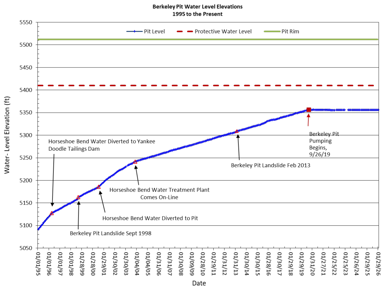
Figure 3-24. Water-level hydrograph of the Berkeley Pit, 1995–2025.
