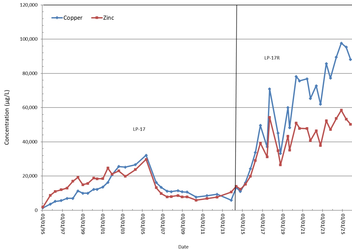
Figure 2-17. Copper and zinc concentrations in wells LP-17 and LP-17R.
