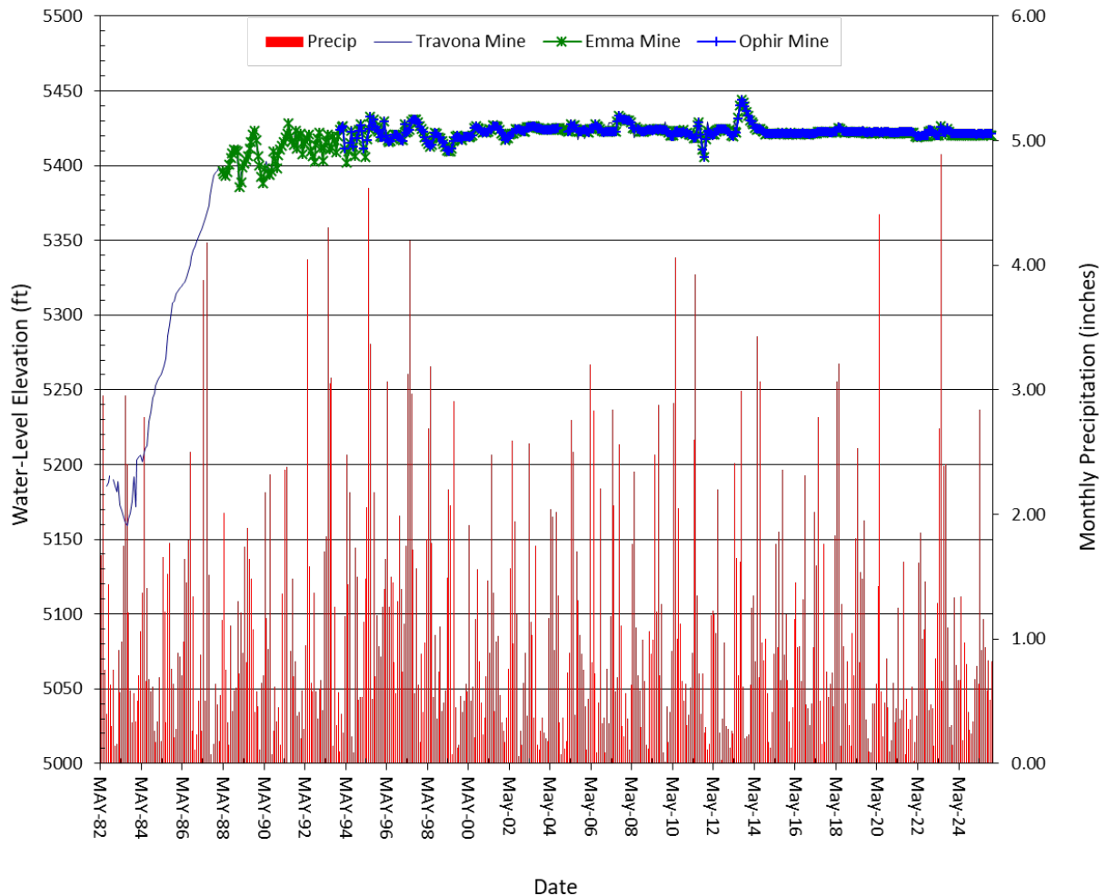
Figure 4-8. Water-level hydrographs for West Camp mines compared to monthly precipitation.
