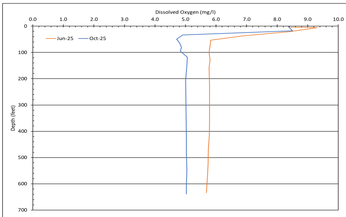
Figure 3-34. Berkeley Pit 2025 dissolved oxygen profiles.
