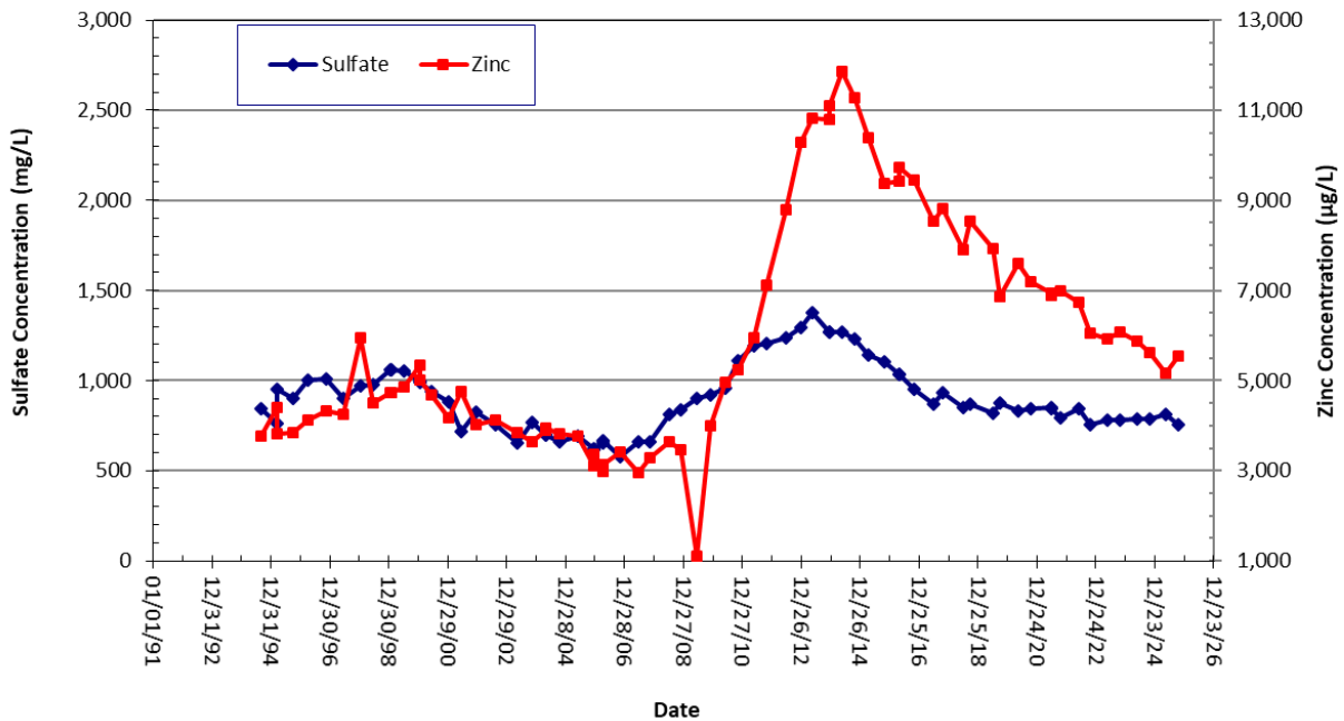
Figure 2-16. Sulfate and zinc concentrations in well LP-16.
