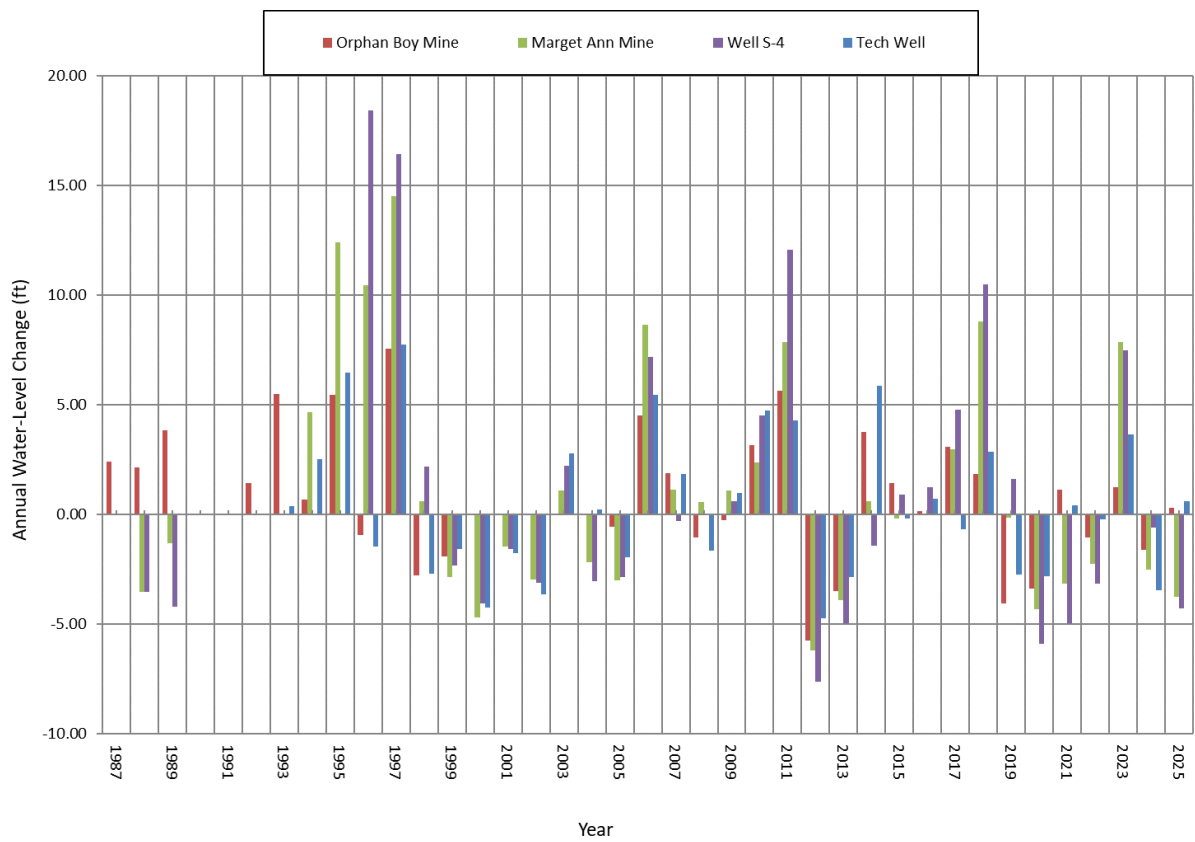
Figure 5-2. Outer Camp sites annual water-level change.
