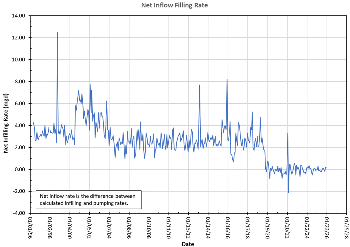
Figure 6-2. Berkeley Pit net filling rate, 1996–2025.
