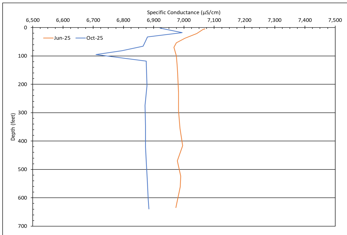
Figure 3-32. Berkeley Pit 2025 specific conductance profiles.
