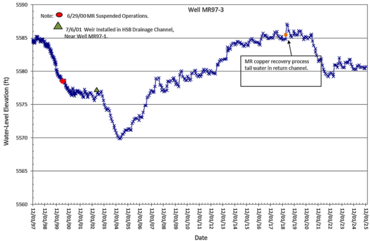
Figure 2-19. Water-level hydrograph for well MR97-3.
