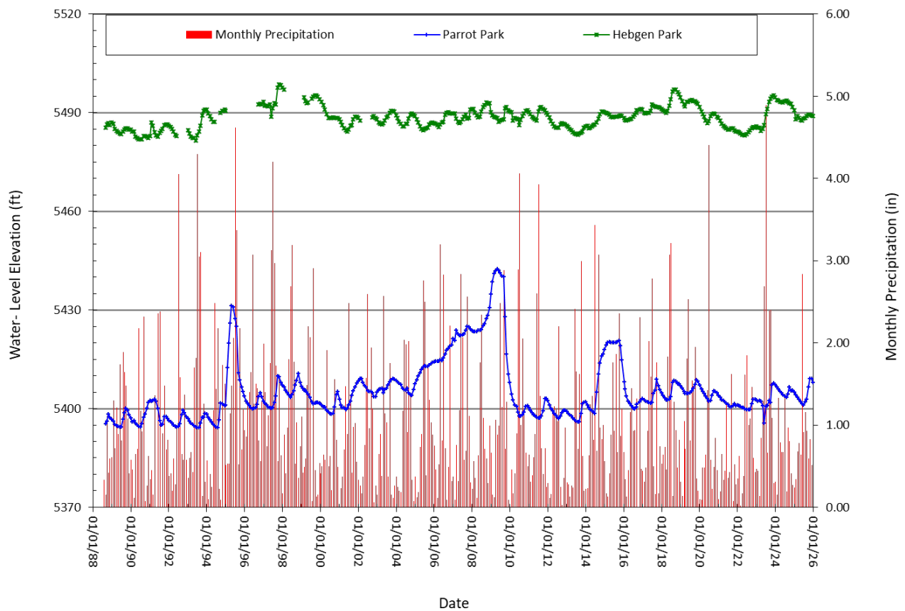
Figure 3-19. Water-level hydrograph for the Parrot Park and Hebgen Park wells.
