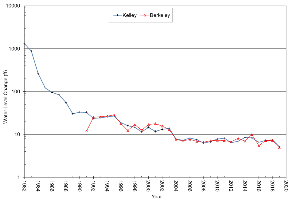
Figure 3-2A. Kelley Mine and Berkeley Pit annual water-level changes, 1982–2020.
