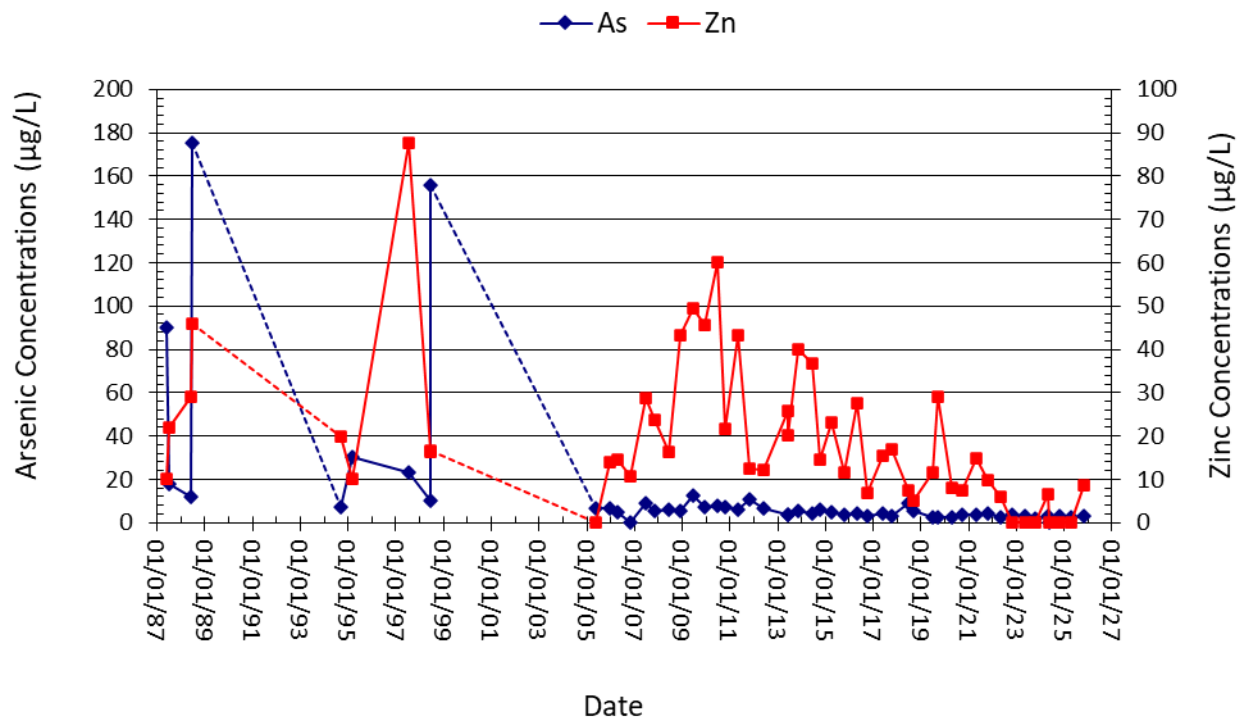
Figure 5-7. Arsenic and zinc concentrations in water sampled from the Orphan Boy mine.
