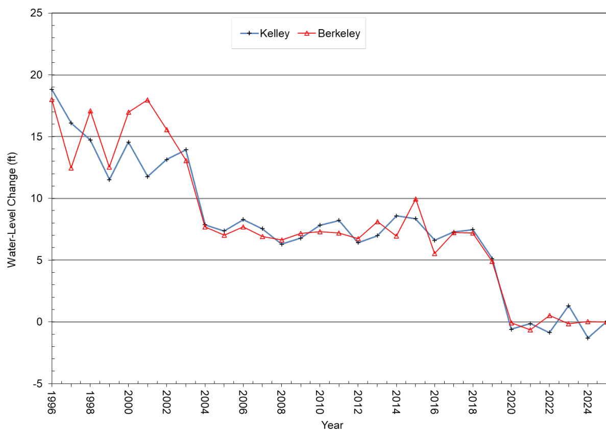
Figure 3-2B. Kelley Mine and Berkeley Pit annual water-level changes, 1996–2025.
