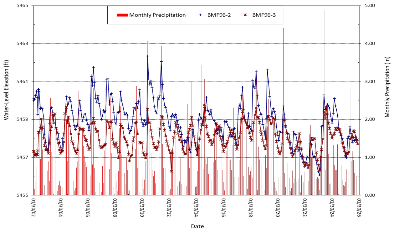
Figure 4-12. Water-level hydrographs for wells BMF96-2 and BMF96-3, 2002–2025.
