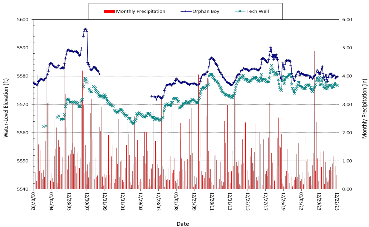
Figure 5-4. Water-level hydrograph for the Orphan Boy Mine and Montana Tech well.
