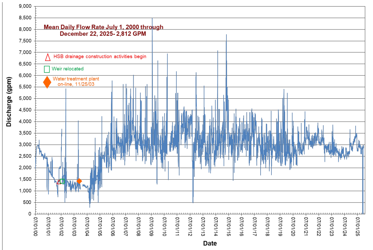
Figure 3-26. Horseshoe Bend Drainage flow rate, July 2000 through December 2025.
