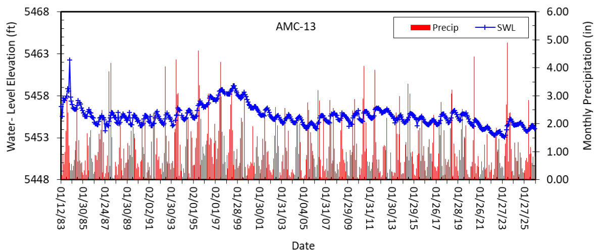
Figure 2-5. Water-level hydrograph for well AMC-13.
