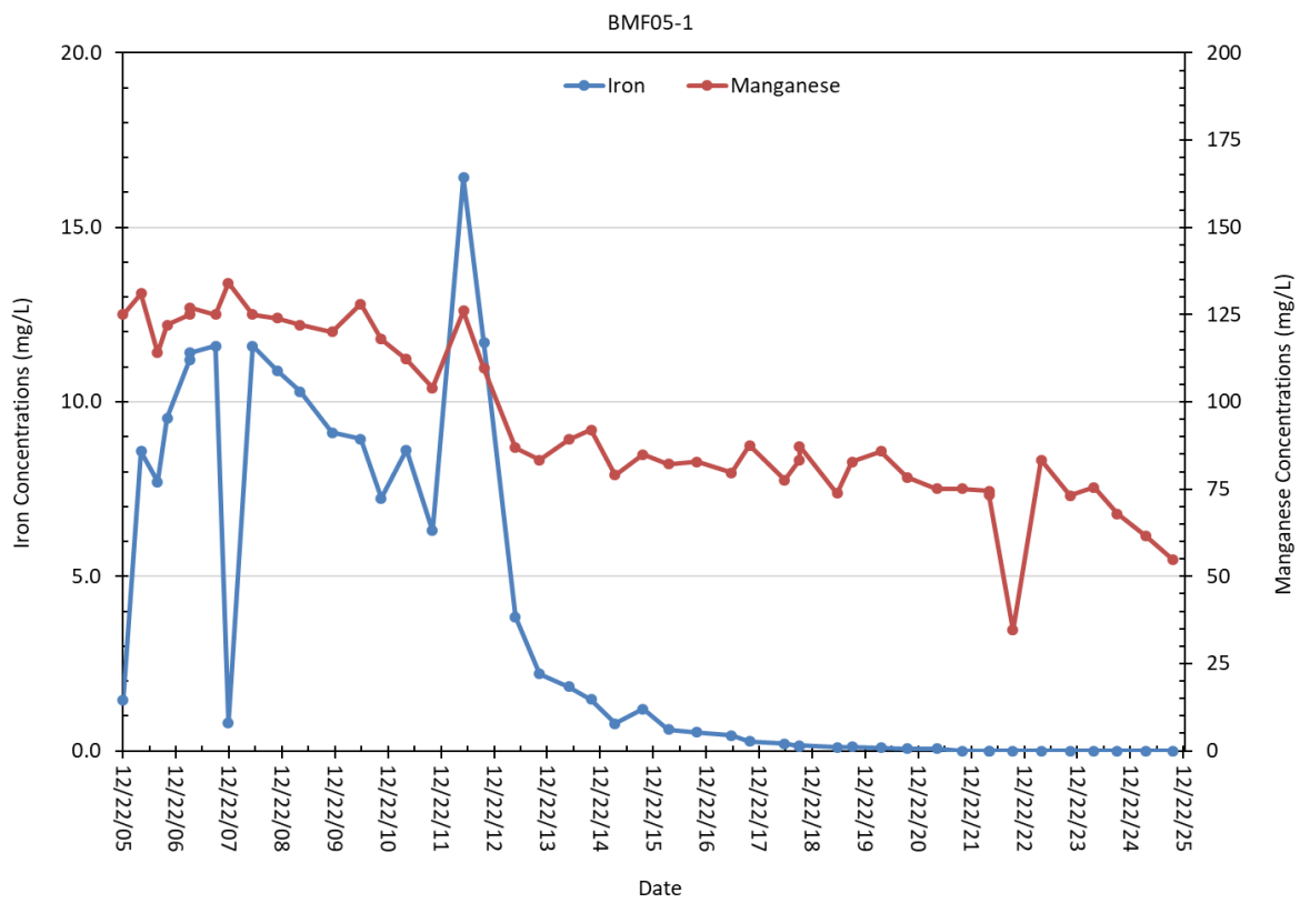
Figure 2-26. Iron and manganese concentration trends in well BMF05-1.
