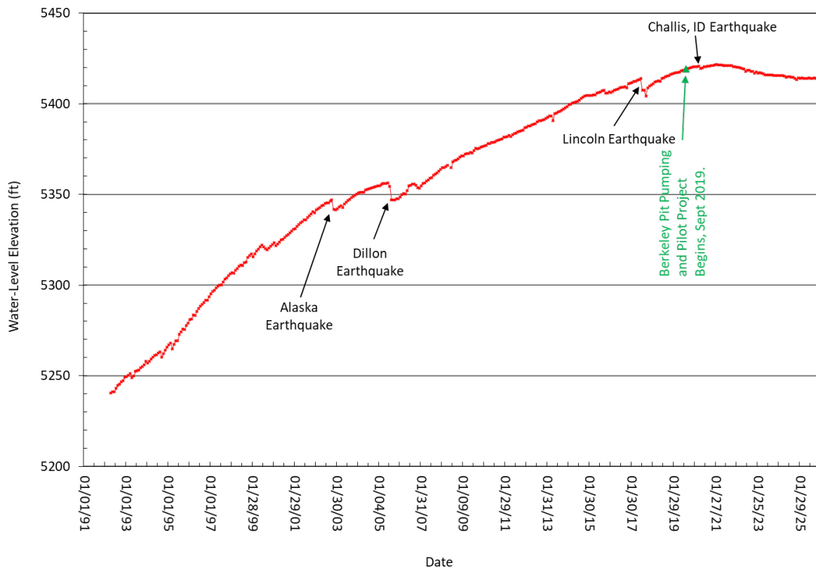
Figure 3-11. Water-level hydrograph for bedrock well B shows water-level response to earthquakes.
