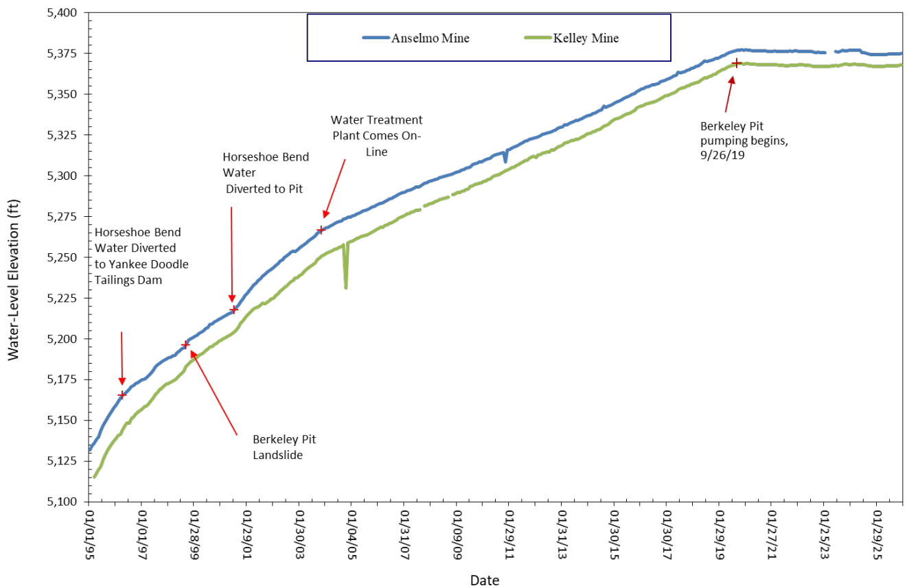
Figure 3-3. Water-level hydrograph for the Anselmo and Kelley mines from 1995 to 2025, and significant events that affected the rate of water-level rise.
