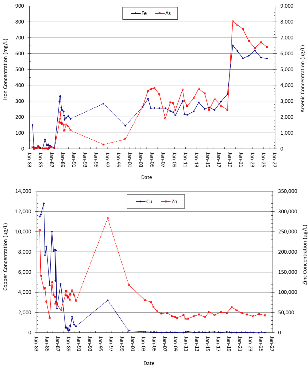
Figure 3-8. Steward Mine iron and arsenic concentrations (top), copper and zinc concentrations (bottom) over time.
