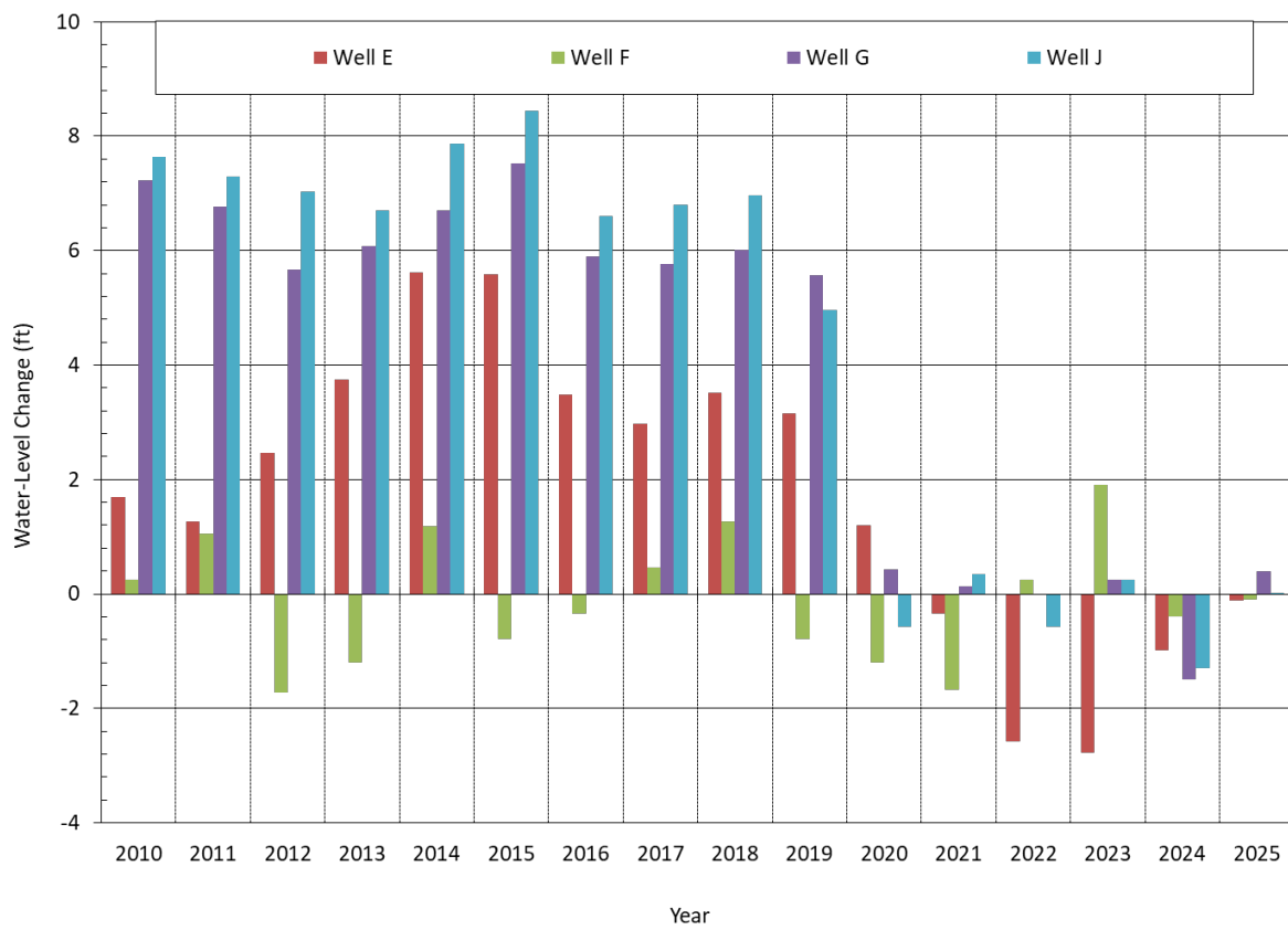
Figure 3-9. Annual water-level change in bedrock wells from 2010 to 2025.
