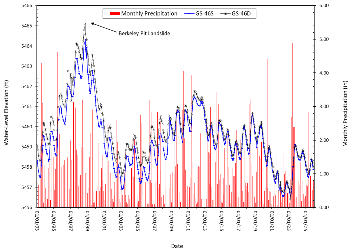
Figure 2-22. Water-level hydrographs for wells GS-46S and GS-46D.
