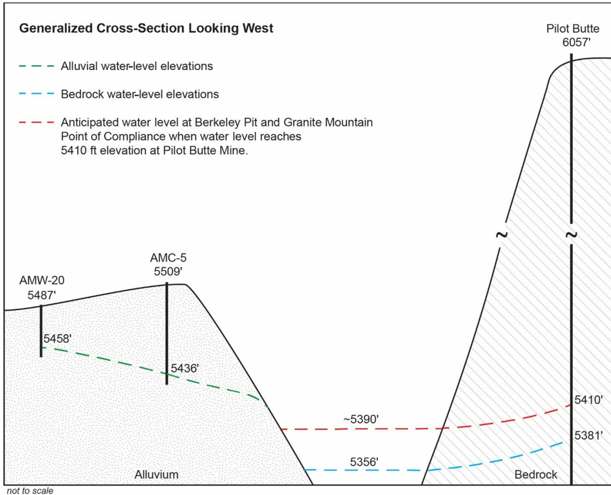
Figure 1-11. Generalized cross-section looking west through the Berkeley Pit depicting water-level elevations in bedrock and alluvial systems in December 2025 and projected elevations when the 5,410 Protective Water Elevation is reached at the Pilot Butte Mine (location shown in figure 1-10).
