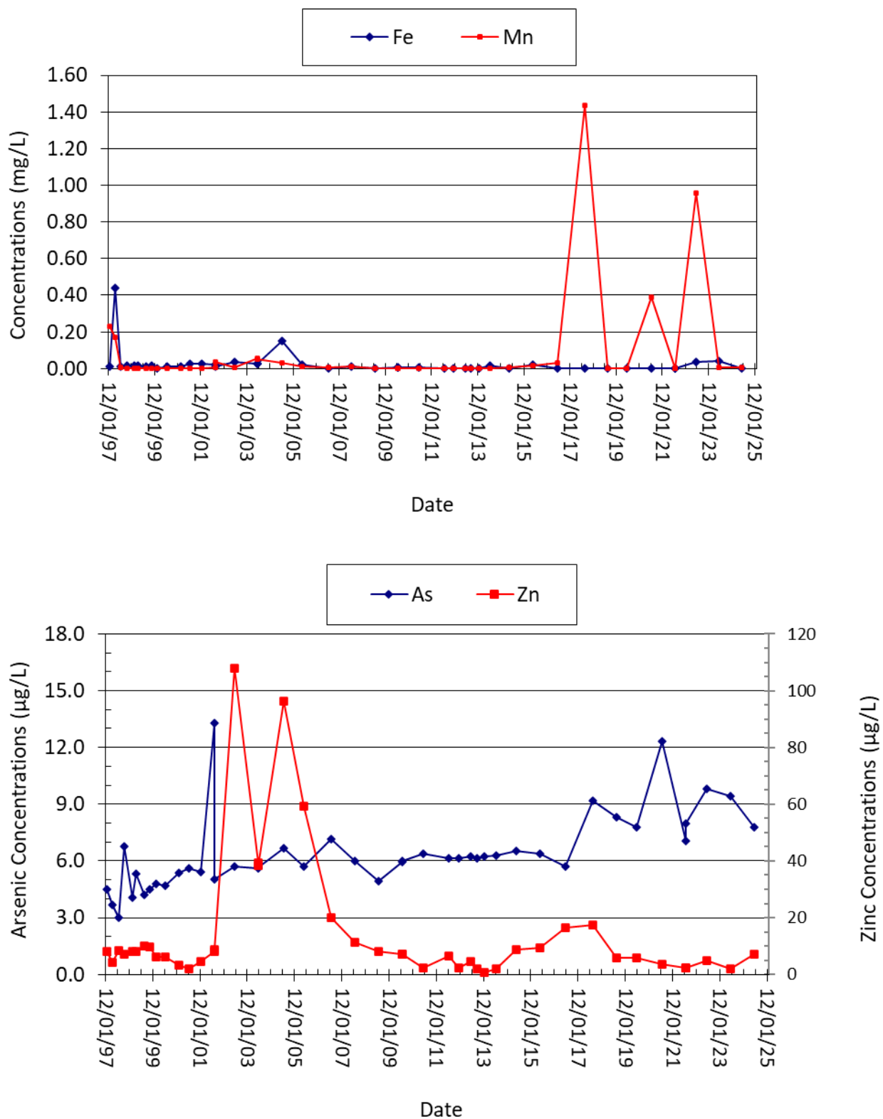
Figure 4-15. Selected water chemistry for West Camp well BMF96-4.
