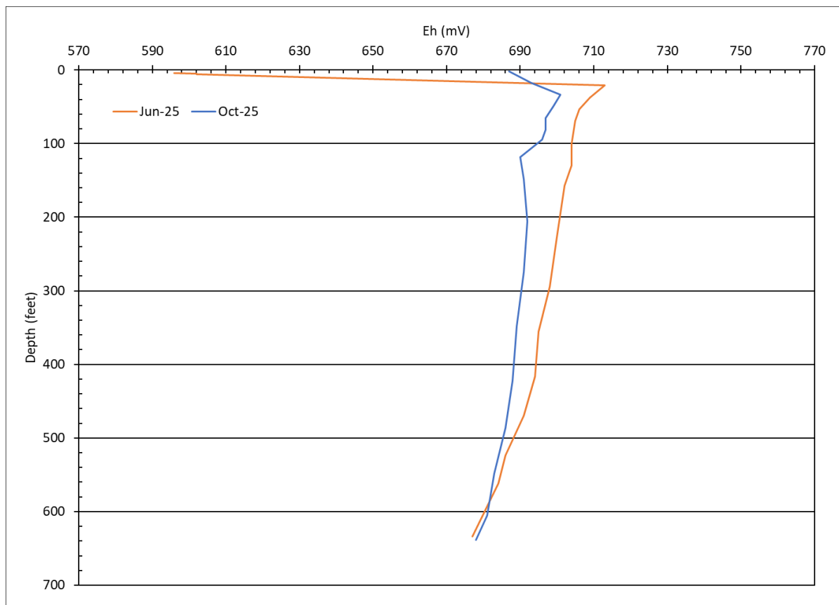
Figure 3-35. Berkeley Pit 2025 oxidation reduction profiles (Eh).
