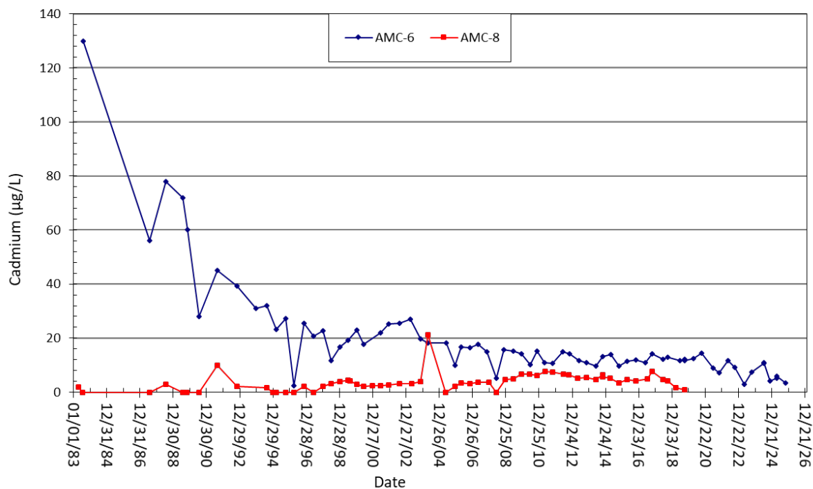
Figure 2-7. Cadmium concentration changes over time for wells AMC-6 and AMC-8.
