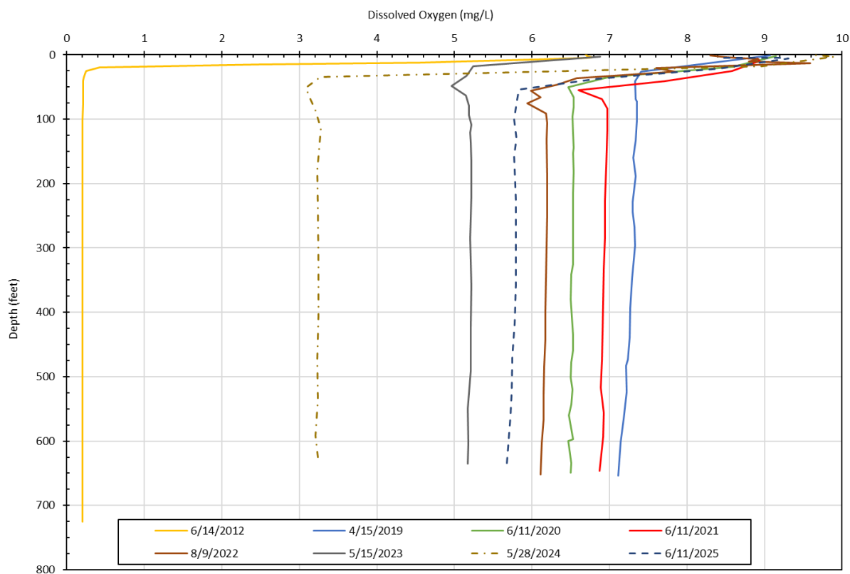
Figure 3-37. Comparison of dissolved oxygen profiles in the pit during spring 2012 and spring 2019–2025.
