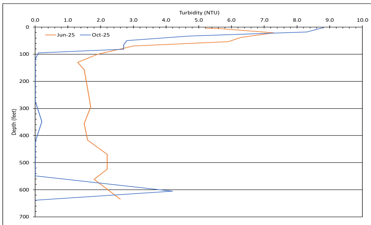
Figure 3-36. Berkeley Pit 2025 turbidity profiles.
