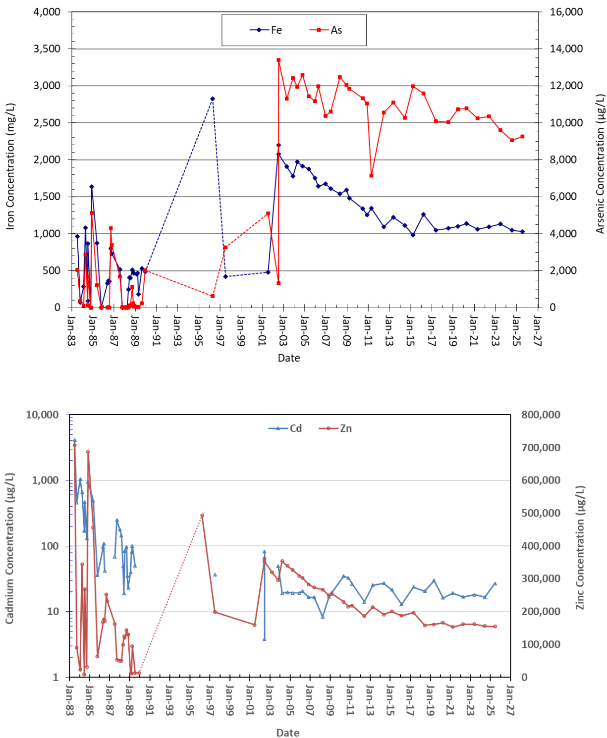
Figure 3-6. Kelley Mine iron and arsenic concentrations (top) and cadmium and zinc concentrations (bottom) over time.
