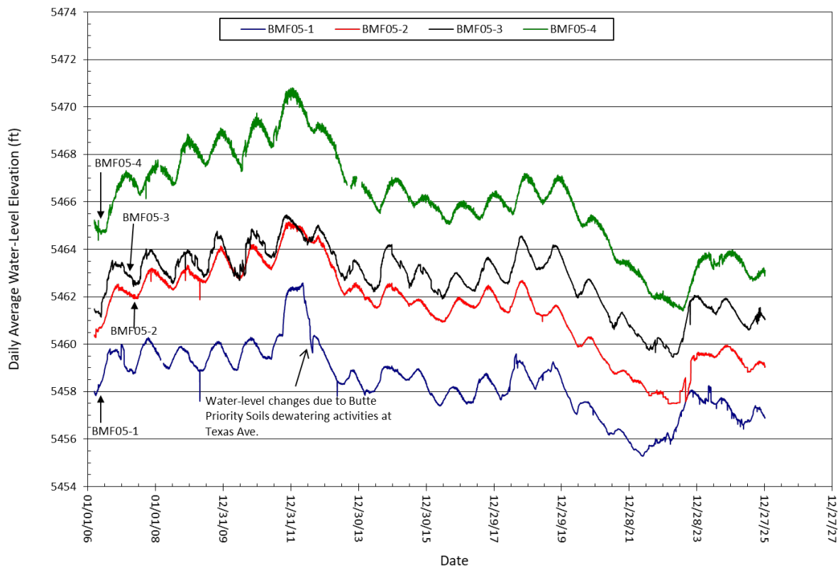
Figure 2-23. Daily average water levels for BMF05-series wells.
