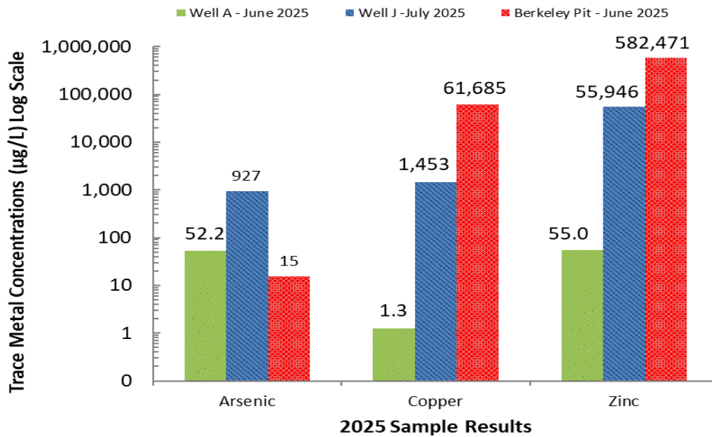
Figure 3-17. Selected trace metal comparisons among bedrock wells A, J, and the Berkeley Pit 4-ft depth sample.
