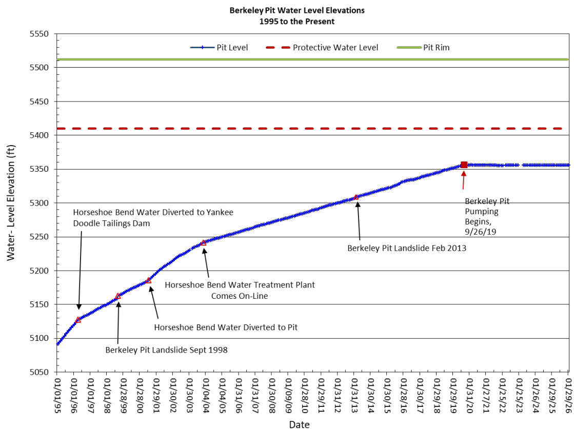
Figure 3-4. Berkeley Pit water-level hydrograph from 1995 to 2025.
