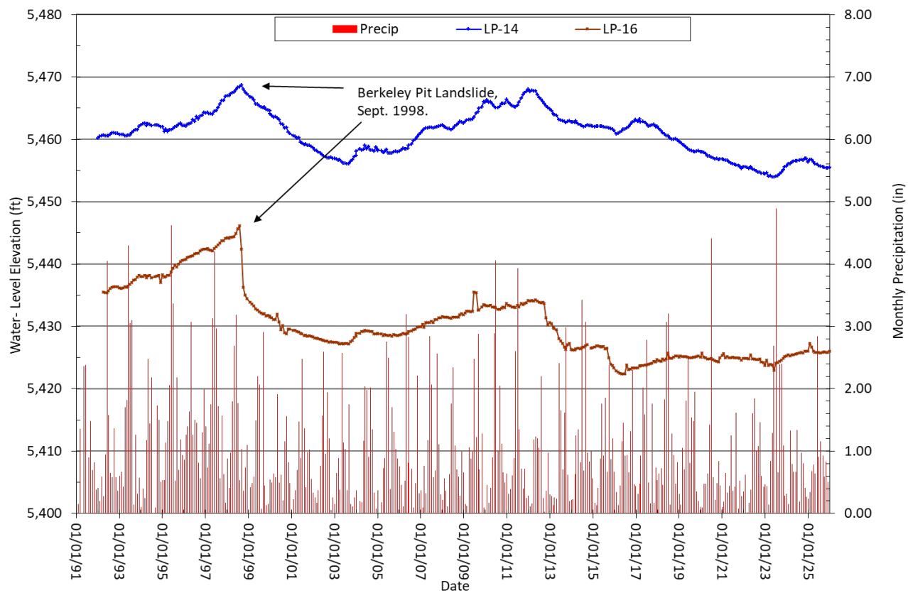
Figure 2-12. Water-level changes for wells LP-14 and LP-16 before and after the 1998 Berkeley Pit landslide.
