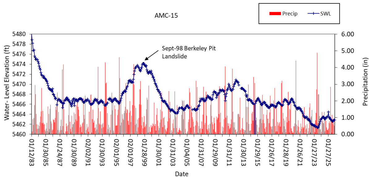
Figure 2-6. Water-level hydrograph for well AMC-15.
