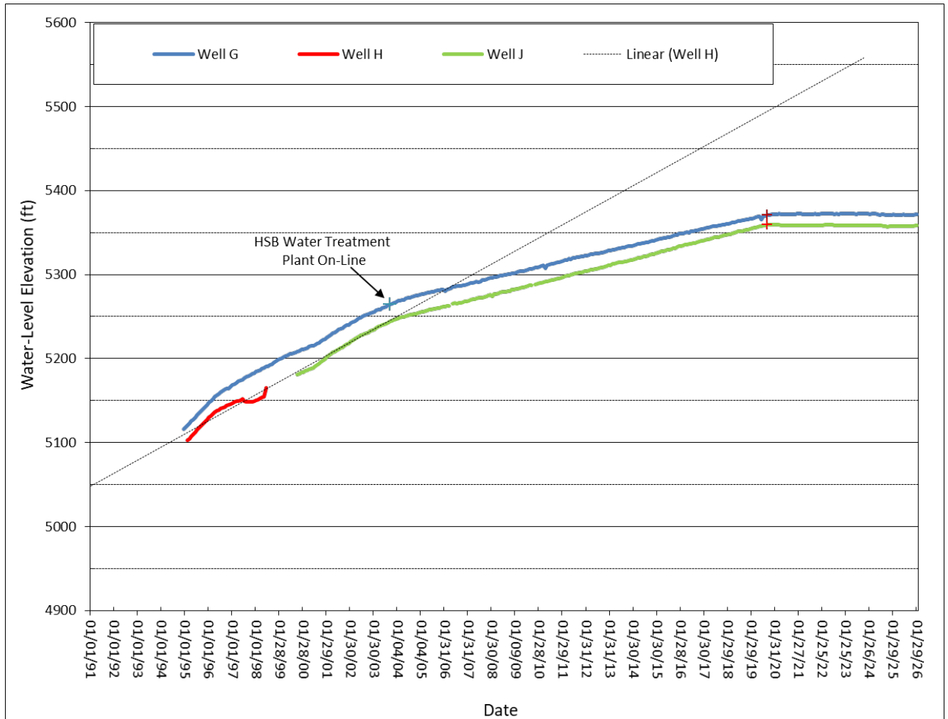
Figure 3-13. Water-level hydrographs for bedrock wells G, H, and J.
