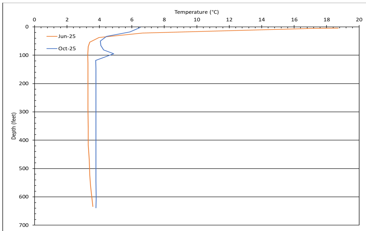
Figure 3-33. Berkeley Pit 2025 temperature profiles.
