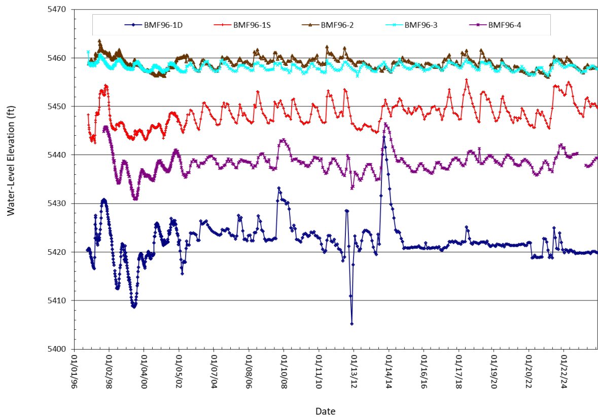
Figure 4-11. Water-level hydrographs for BMF96-series wells, 1996–2025.
