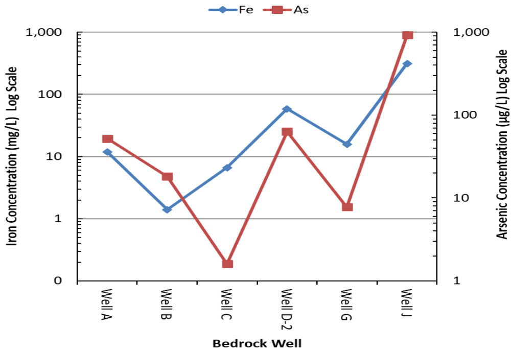
Figure 3-16. Bedrock well iron and arsenic concentration comparisons, spring 2025.
