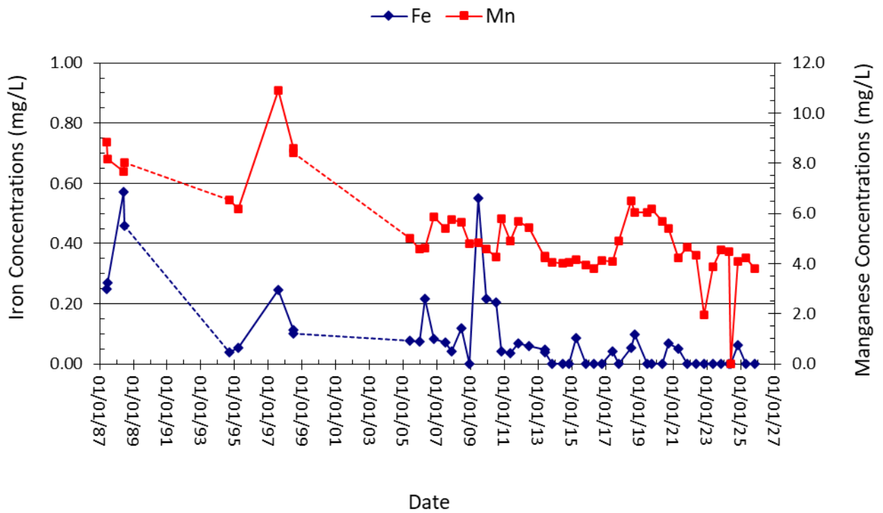
Figure 5-6. Iron and manganese concentrations in water sampled from the Orphan Boy Mine.
