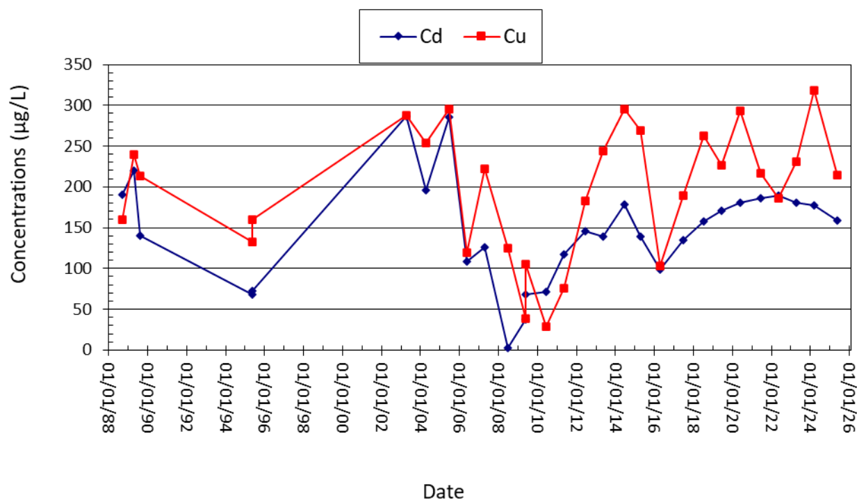
Figure 3-22. Cadmium and copper concentrations for the Parrot Park well.
