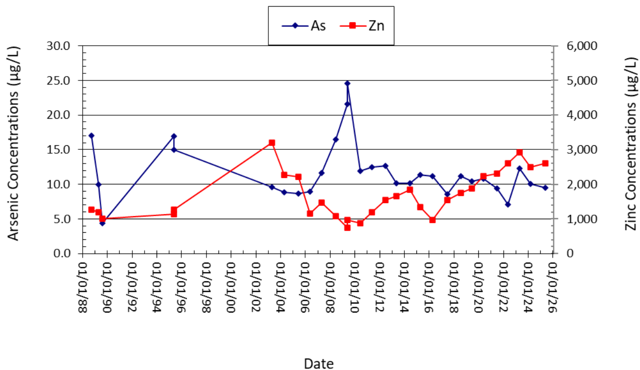
Figure 3-23. Arsenic and zinc concentrations for the Parrot Park well.
