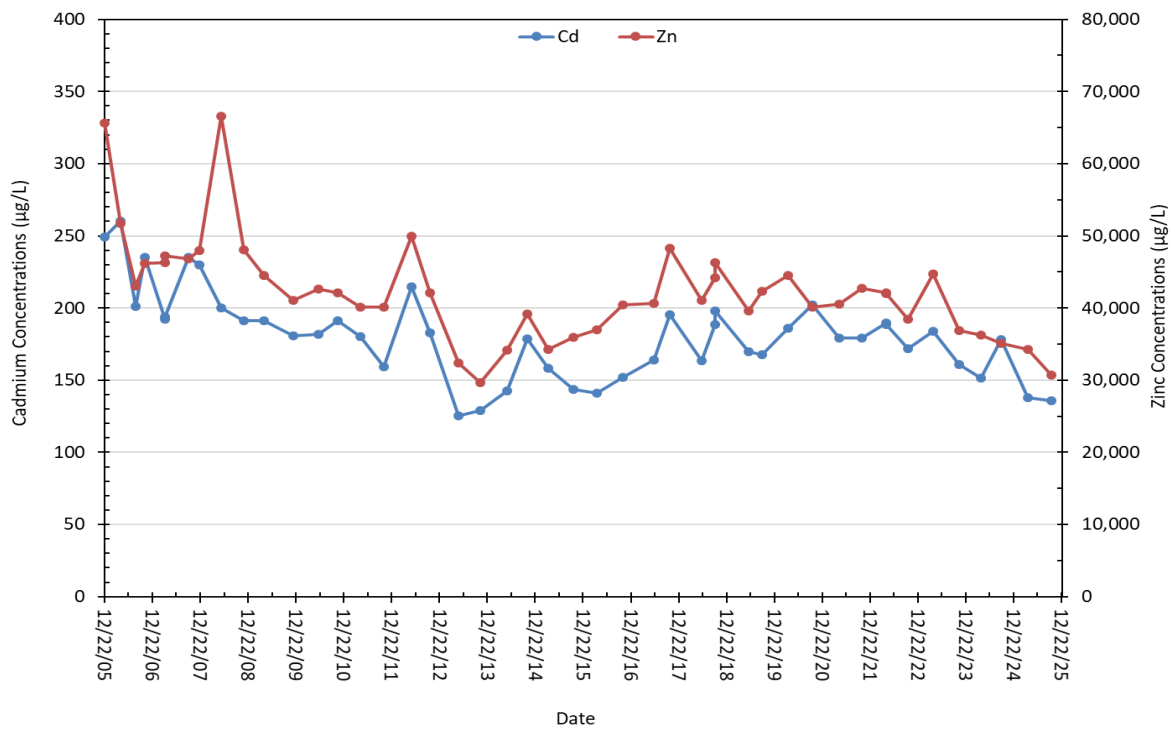
Figure 2-27. Cadmium and zinc concentration trends in well BMF05-1.
