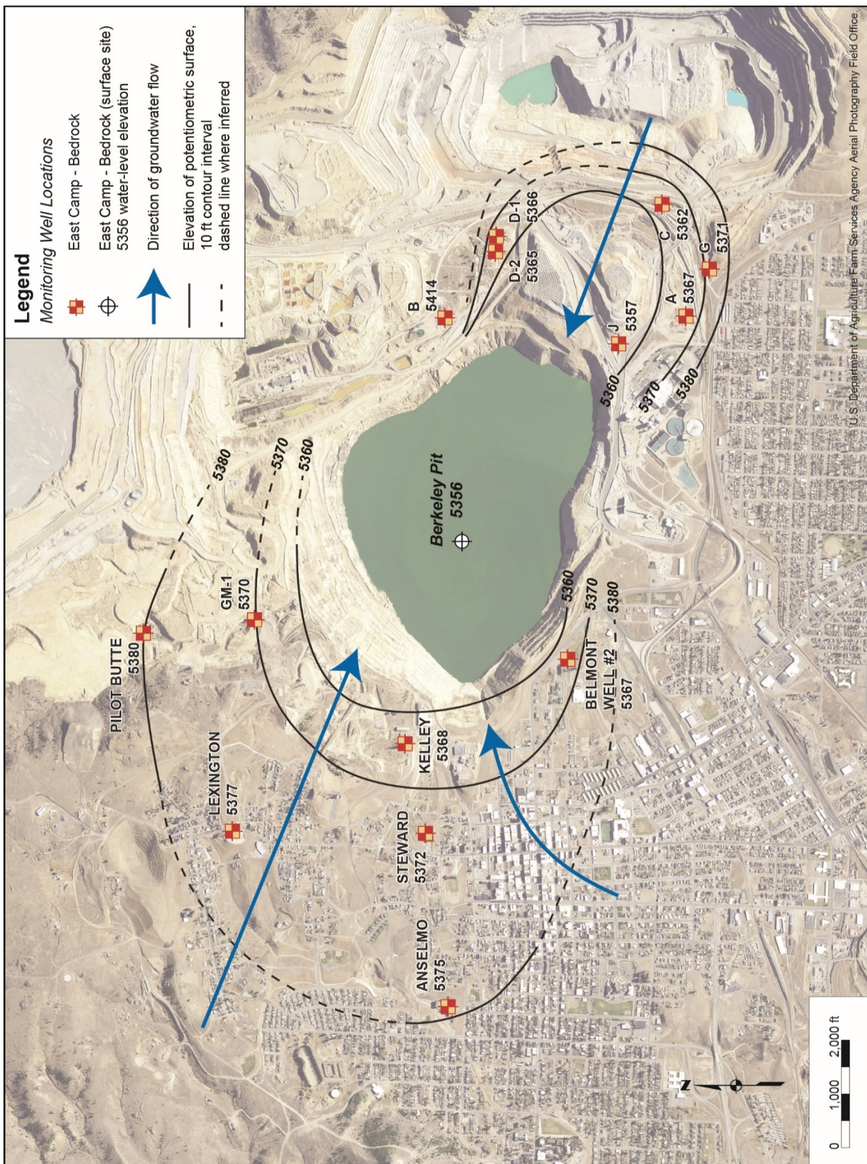
Figure 3-15. Potentiometric map for the East Camp bedrock aquifer, December 2025 (contour interval is 10 ft).
