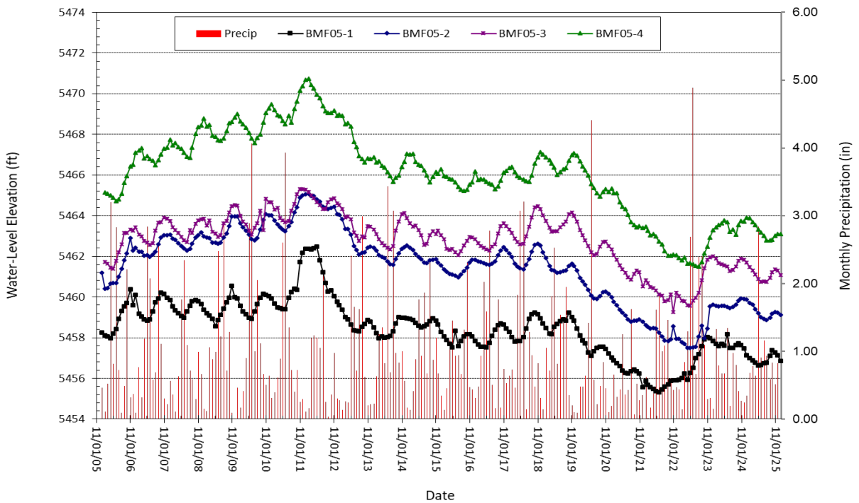
Figure 2-24. Monthly water levels versus precipitation, BMF05-series wells.
