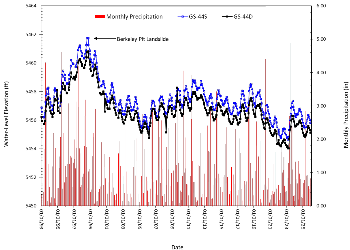
Figure 2-21. Water-level hydrographs for wells GS-44S and GS-44D.
